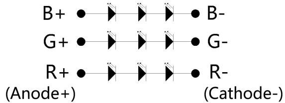
Circuit diagram
